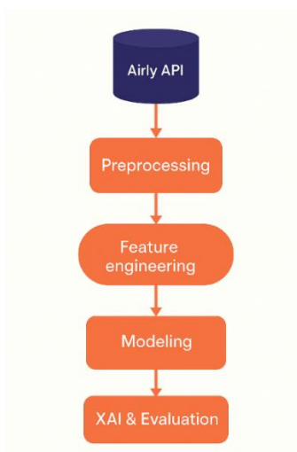
Fig. 1. Overview of the ML data pipeline used in this research.
