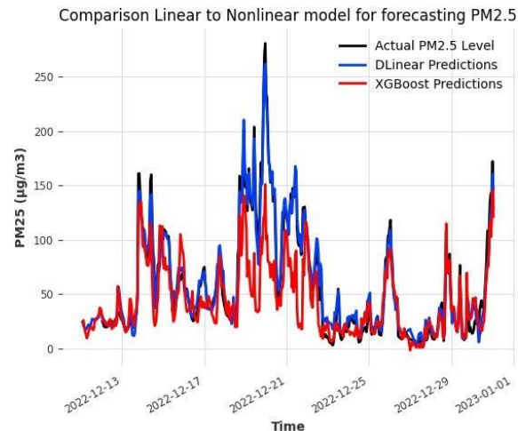
Fig. 7. Evaluation of XGBoost and DLinear for PM 2.5 forecasting.
